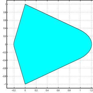
Figure 3: The imaginary numbers i and -i (corners) must be eigenvalues.
